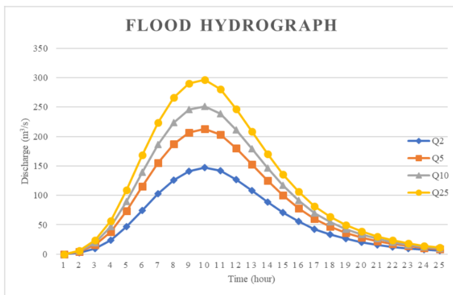
Figure 3. Flood Hydrograph
